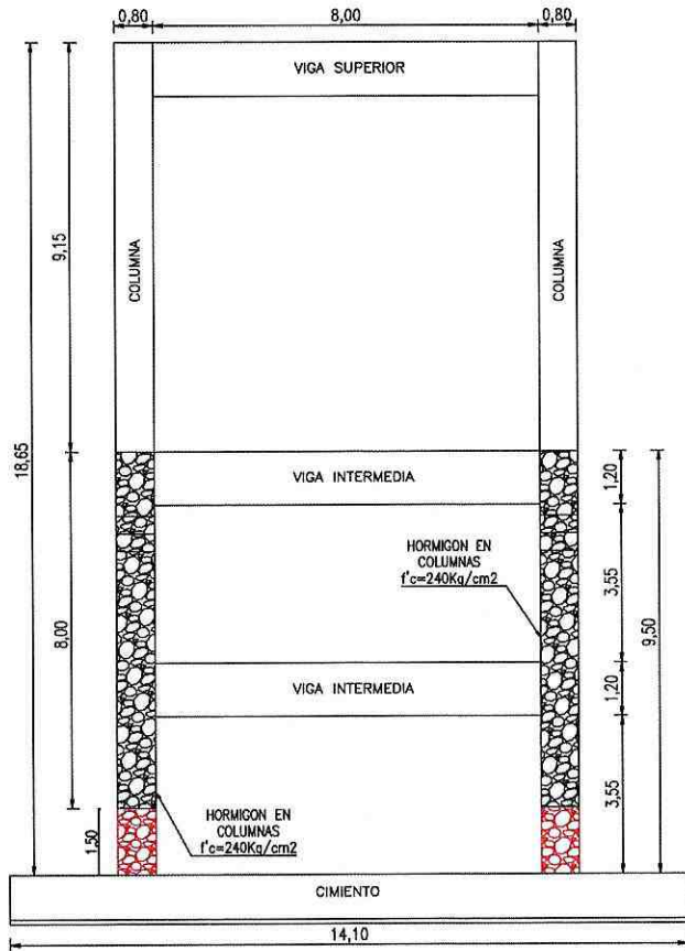
VISTA FRONTAL
