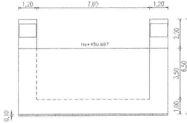
VISTA FRONTAL
